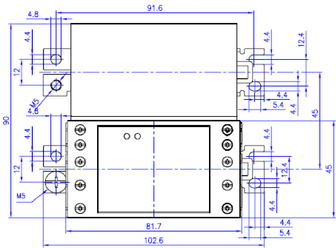
WITH M5 EARTH TERMINATION BOLT
